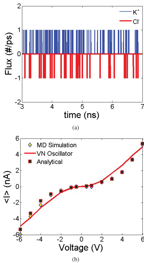
Fig. 2 (a) Flux of single ion transport inside graphene nanopore. Either one Potassium or Chloride ion transports through the pore at a given time. (b) Current-Voltage characteristics of single ion transport. The region where the current is blocked is called Coulomb blockade region and region where current flows is called single ion transport region. Comparison of MD (diamond symbols), VN oscillator model (solid line) and analytical (filled squares) results
