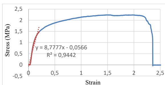
Fig. 4 Stress-Strain Diagram, with cross-linking. Young's modulus= 8.8 ±/ 0.6 MPa, \epsilon^{UTS} = 2.23 ±/ 0.022, strain at break= 200%
