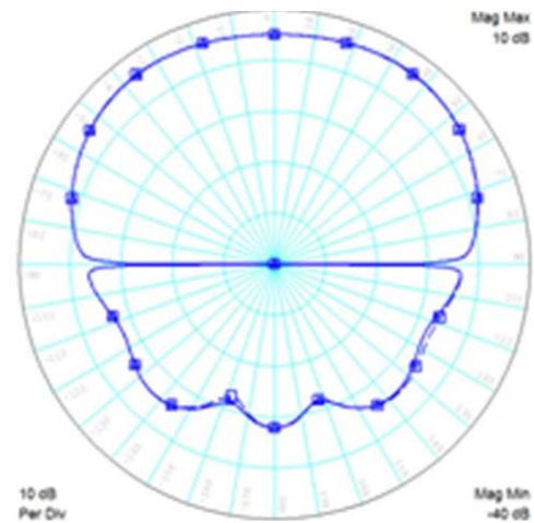
Fig. 5 Dual Polarization antenna for 28 GHz. Radiation pattern of the antenna (solid line – XZ plane and dashed line – YZ plane). The directivity is 5.0dBi
