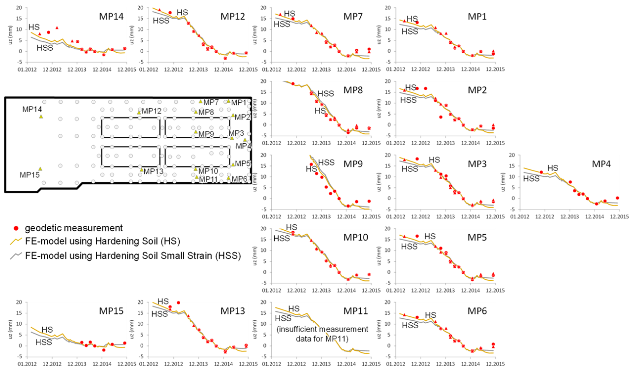
Fig. 7 Measurements and modelled behaviour (settlements vs time)
