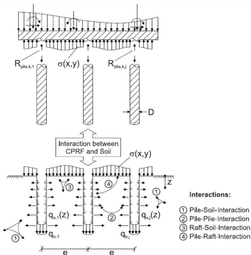
Fig. 1 Behaviour of Piled Raft Foundation [9]
