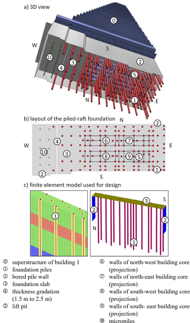
Fig. 5 Foundation layout and numerical modelling
