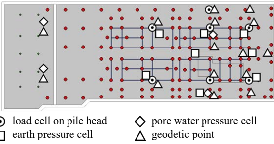
Fig. 6 Monitoring instrumentation
