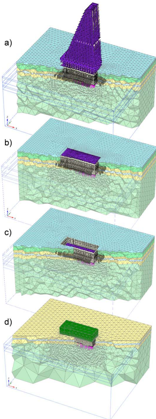
Fig. 2 Modelling of piled raft foundation
