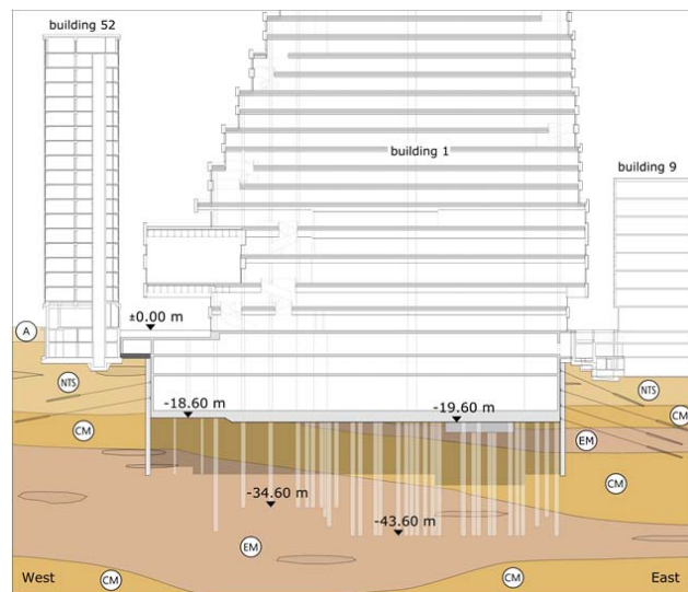
Fig. 4 Geological section (West - East)
