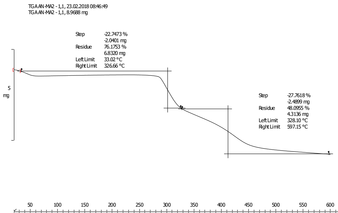
Fig. 5 TGA curves of P(AN-MA)2 copolymer
