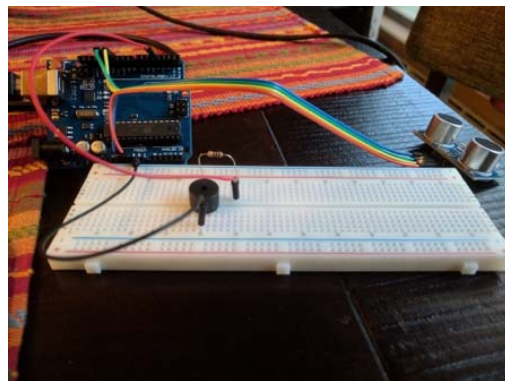
Fig. 5 Microcontroller board connections
