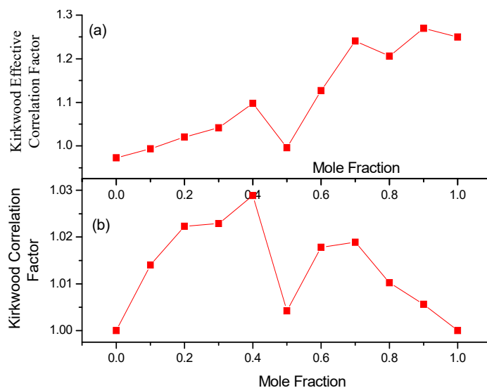
Fig. 3 (a) Kirkwood effective correlation factor ( g^{\text{eff}} ), (b) Kirkwood correlation factor ( g_f ) versus mole fraction ( \Phi_2 ) of DMF in DE at 10°C temperatures
