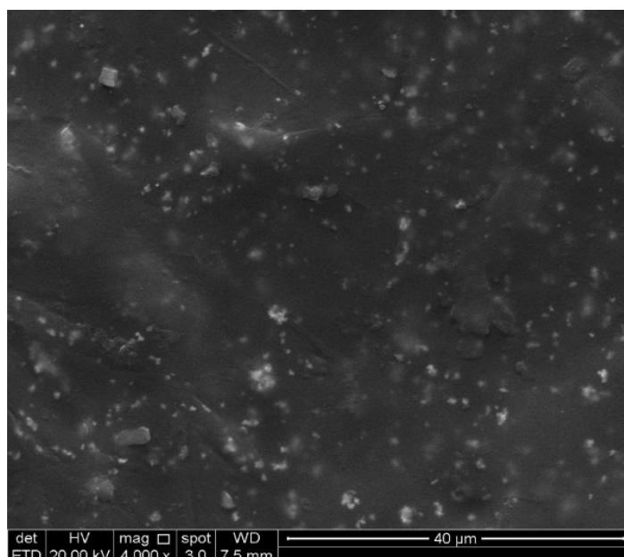
Fig. 1 (a) SEM of \text{Bi}_2\text{O}_3 /epoxy-PVA nanofibers, using 0.84 mm ID of needle
