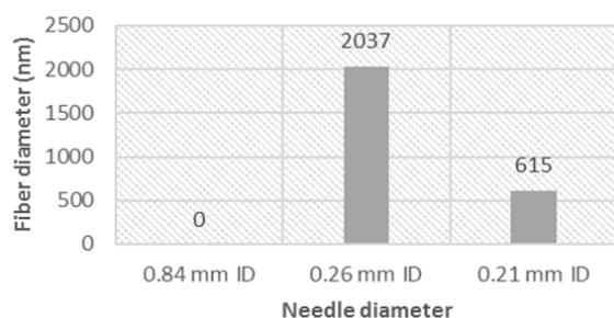
Fig. 2 Needle diameter and average nanofiber diameter obtained
