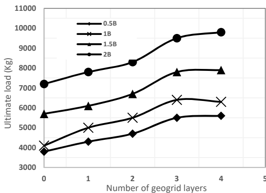
Fig. 10 The ultimate bearing capacity versus the number of geogrid layers for different double-layer soils
