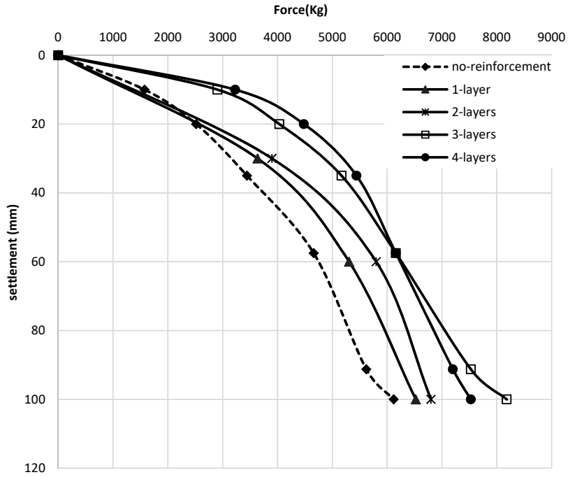
Fig. 4 The influence of number of geogrid layers on the bearing capacity obtained from the plate loading test in a double-layer soil with a top layer thickness (gravel) of 1.5B
