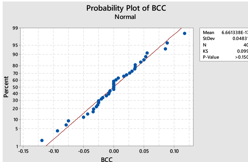
Fig. 1 Results of normality test for BCC model
