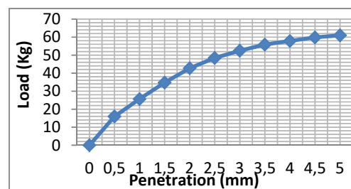
Fig. 3 Load penetration curve
