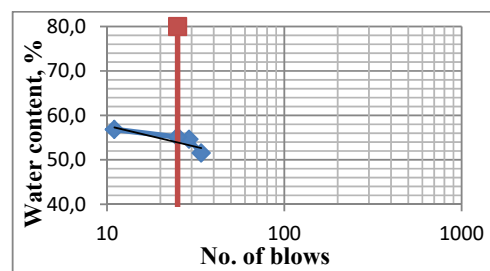
Fig. 2 Flow curve
