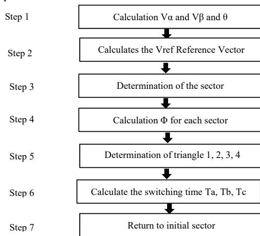
Fig. 6 Steps of the SVPWM
