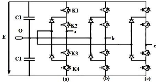
Fig. 1 Three level diode clamped multilevel inverter
