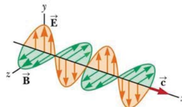
Fig. 1 An electromagnetic wave
