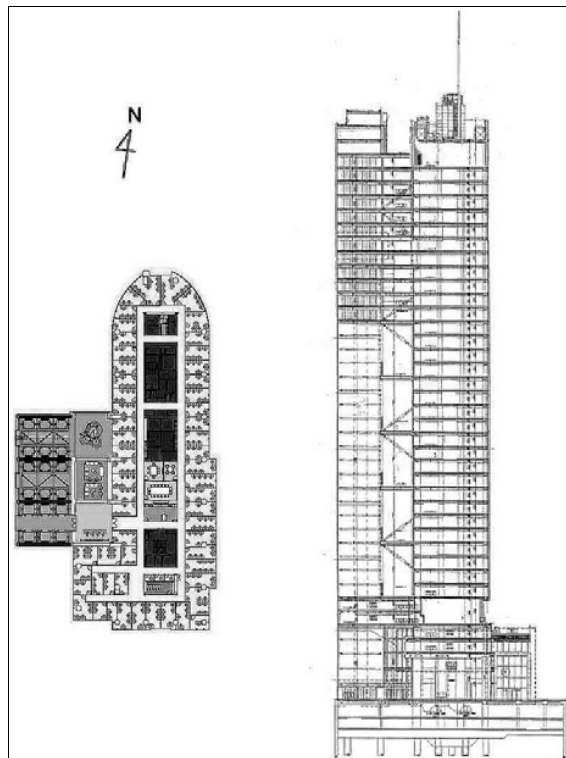
Fig. 6 Rondo 1 Tower: floor plan and section
