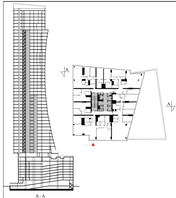
Fig. 10 Złota 44 Tower: floor plan and section
