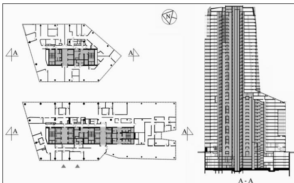
Fig. 14 The Q22 Tower: floor plans and section
