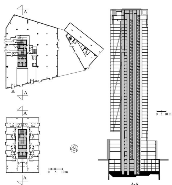
Fig. 8 Cosmopolitan Tower: floor plans and section
