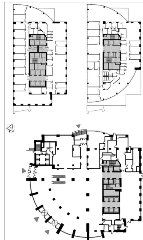
Fig. 4 Warsaw Trade Tower: floor plans
