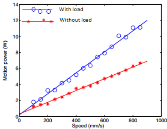
Fig. 5 Power (W) required to use the 'Motion' component when driving the robot at various speeds and different 'loads' [19]
