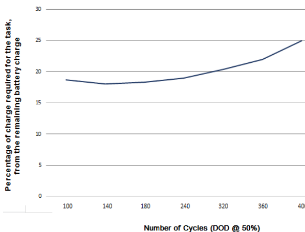
Fig. 4 The percentage charge required to complete a task at various battery cycle stages (DOD set at 50%)
