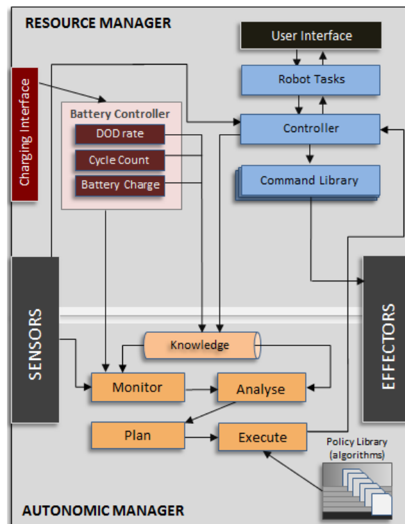
Fig. 3 Autonomic Battery Manager Model
