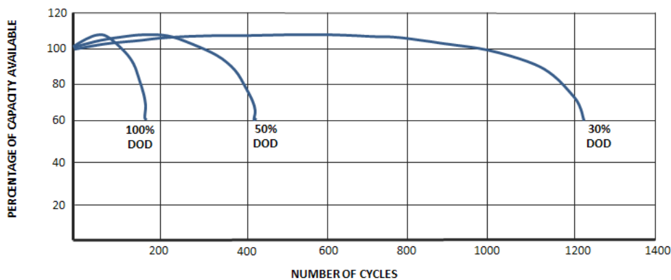
Fig. 1 Shows the DOD characteristics for the lead-acid battery used in the Pioneer 3-AT
