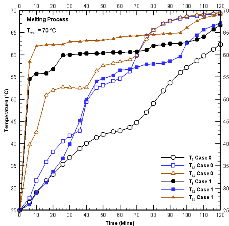
Fig. 5 Temperature comparison for different three cases
