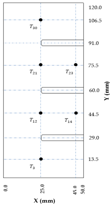
Fig. 1 Schematic of fins integrated LHTES and thermocouples locations [14]
