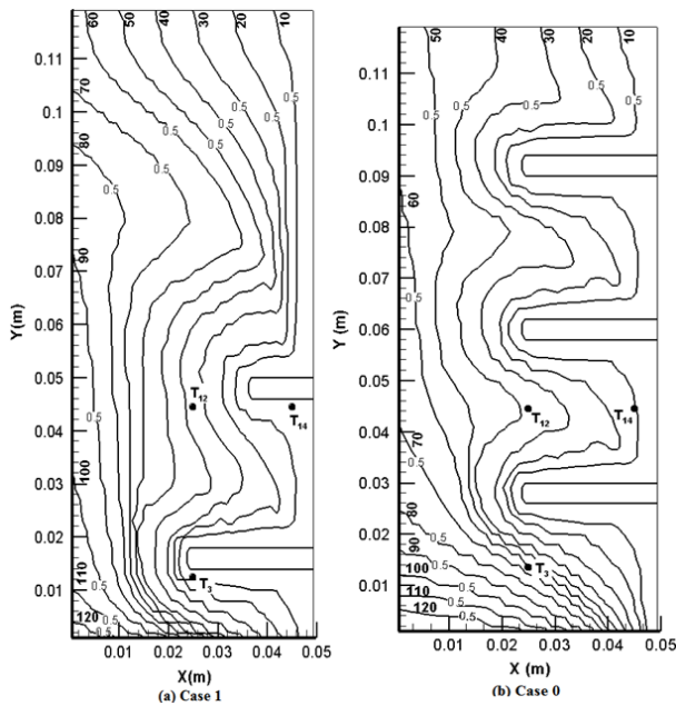
Fig. 4 Comparison between phase front evolutions over time
