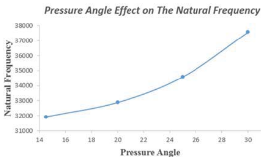
Fig. 19 Pressure angle- natural frequency curve
