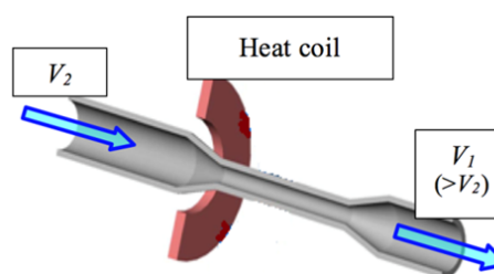
Fig. 1 Schematic illustration of dieless drawing
