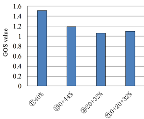
Fig. 4 GOS value for different drawing passes
