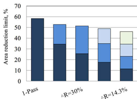
Fig. 5 Relationships between drawing cycle and area reduction limit
