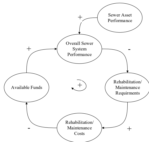
Fig. 1 Reinforcing loop
