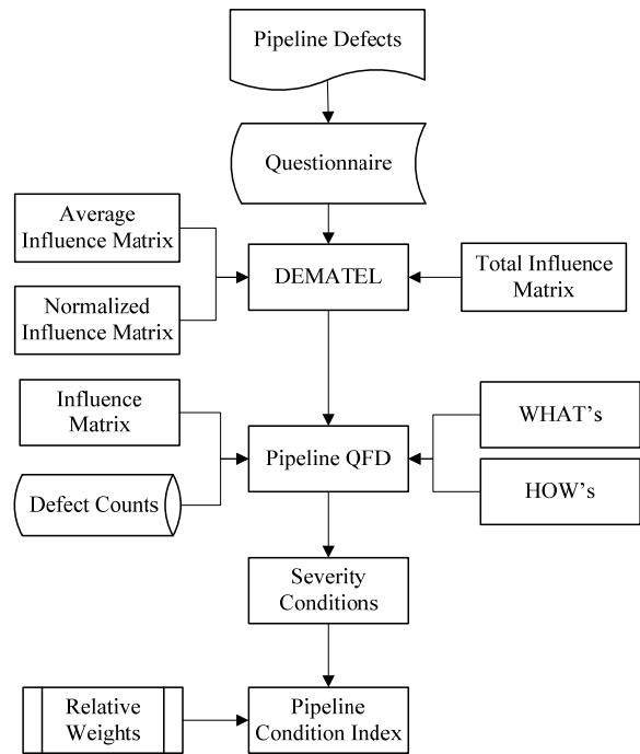
Fig. 4 Proposed methodology
