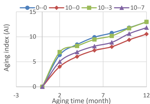
Fig. 8 The variation on the aging index of field specimens
