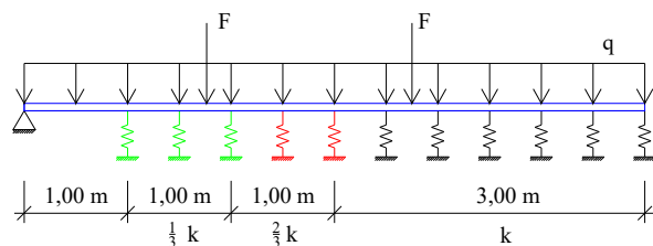
Fig. 3 Model of approaching slab settled on continuous elastic support subjected to equally distributed dead load ( q ) and concentrated ( F ) forces
