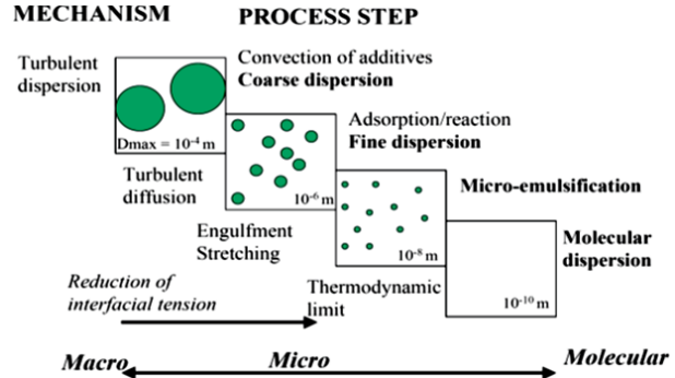
Fig. 2 Schematic of Micro emulsion production [25]
