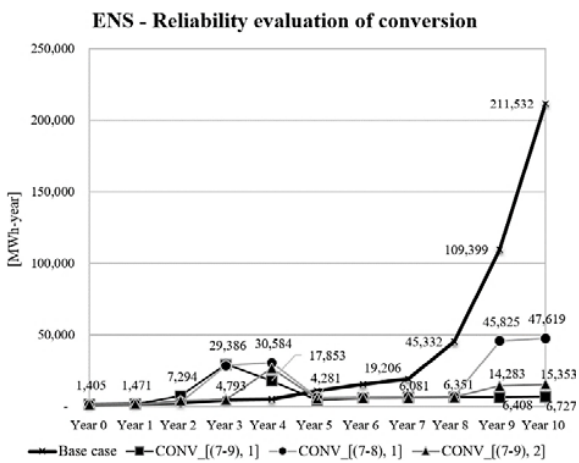
Fig. 7 Assessment of ENS for the base case and conversion alternatives
