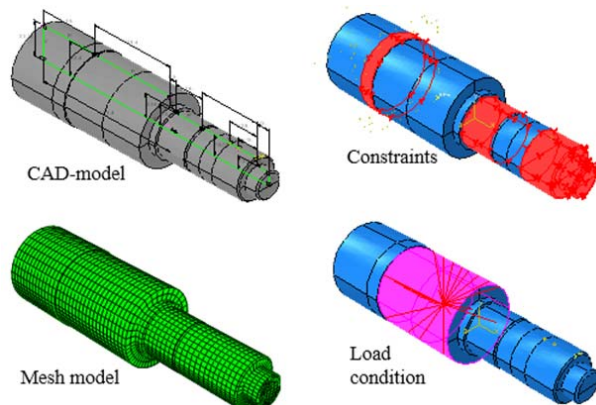
Fig. 5 Shaft modeling
