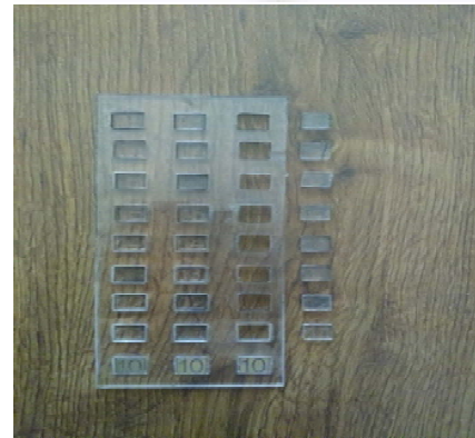
Fig. 2 The produced parts and holes after laser cutting
