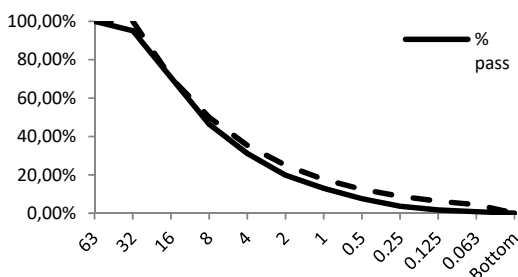
Fig. 1 Particle size distribution of recycled aggregates compared to Fuller's curve
