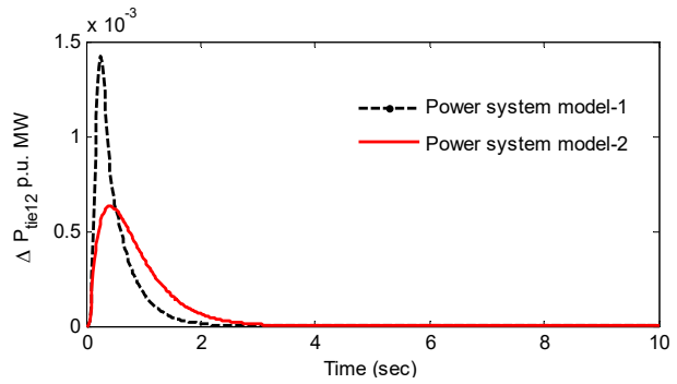
Fig. 5 Response of \Delta P_{tie12} for 1% load disturbance in area-2
