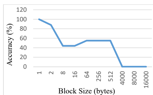
Fig. 2 Change in accuracy according to block size
