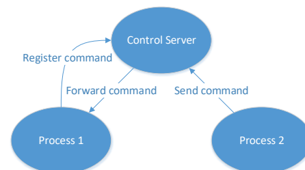
Fig. 5 The DIALOG command diagram
