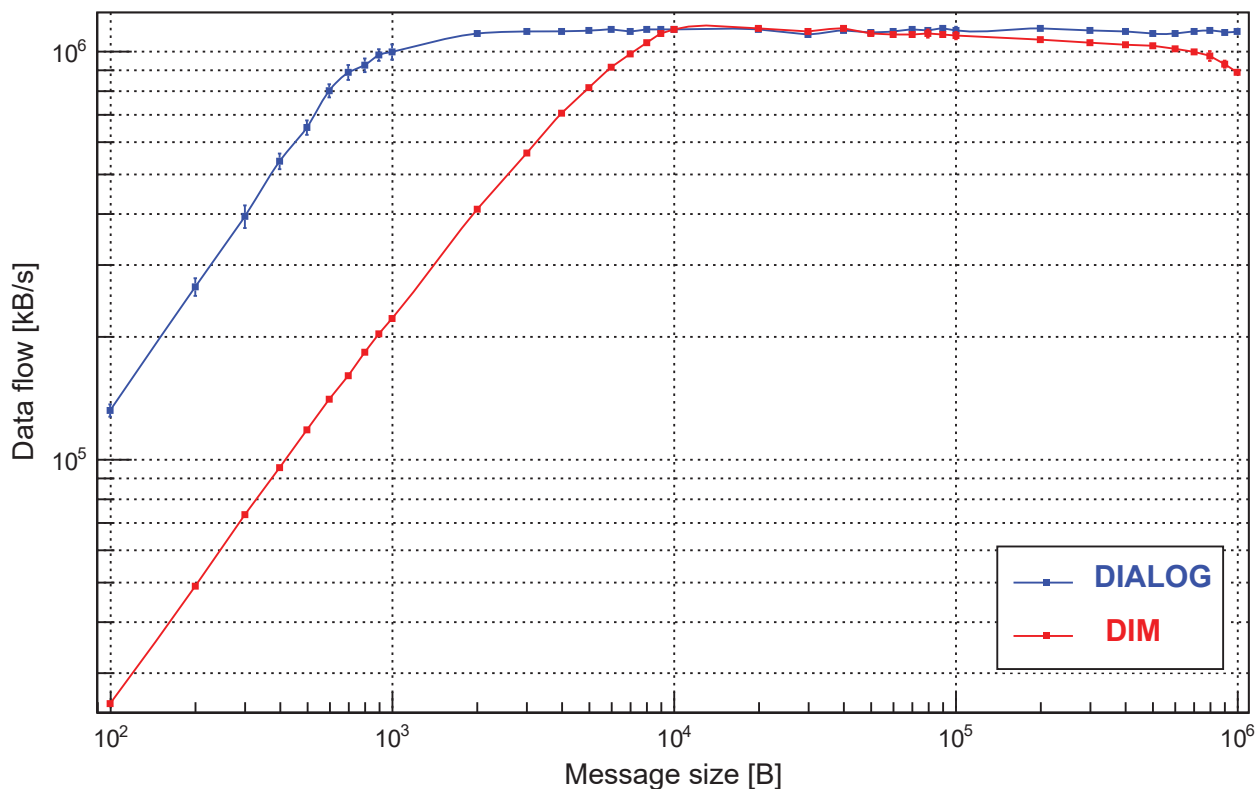
Fig. 10 Data flow
