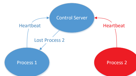
Fig. 4 The DIALOG heartbeats diagram
