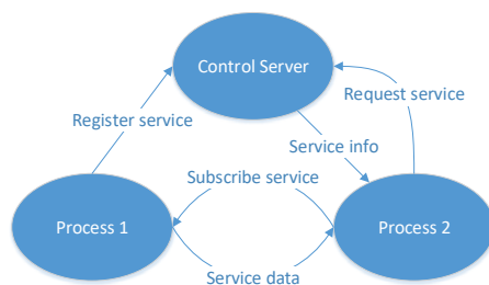
Fig. 7 The DIALOG service diagram
