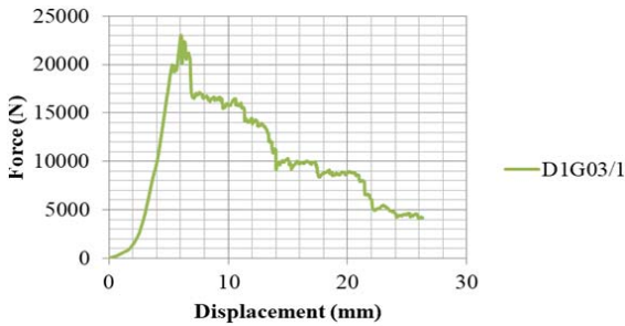
Fig. 11 Force-displacement diagram of the D1G03-1
