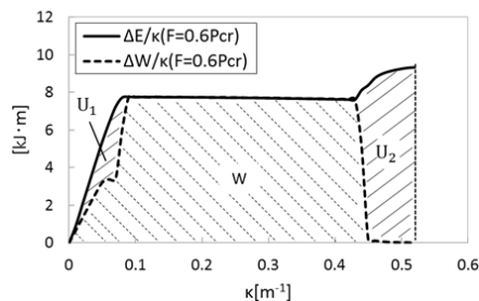
Fig. 20 Comparison energy between F=0,2P cr and F=0,6P cr
