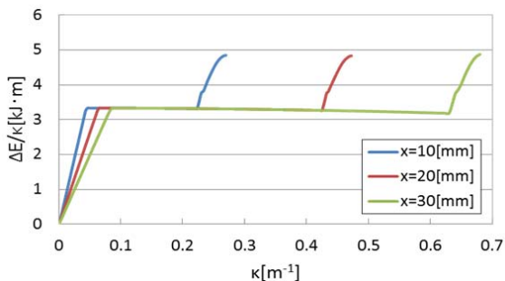
Fig. 21 Energy characteristic due to change x amount
