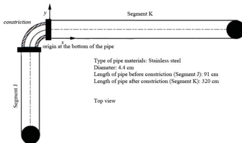
Fig. 8 Constriction location
