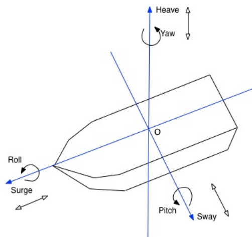
Fig. 1 Ship motion in six DOFs
