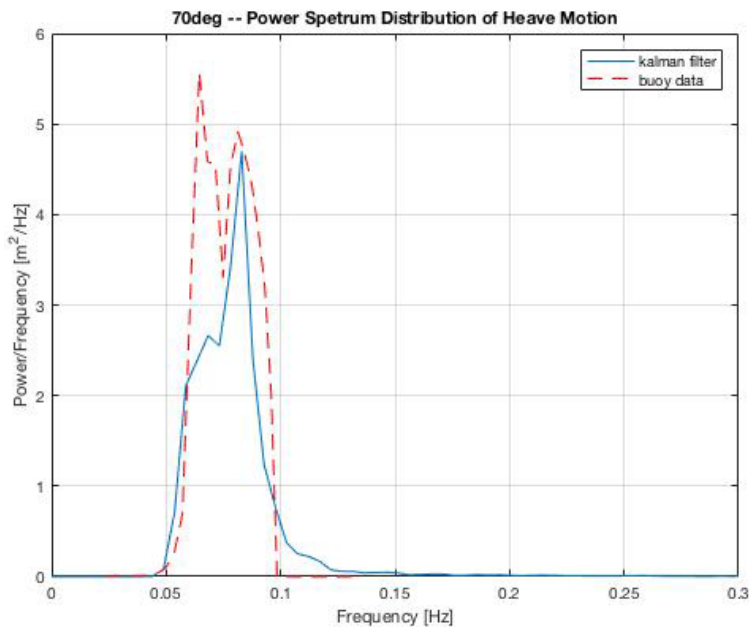
Fig. 6 Heave motion PSD at heading angle of 70°
