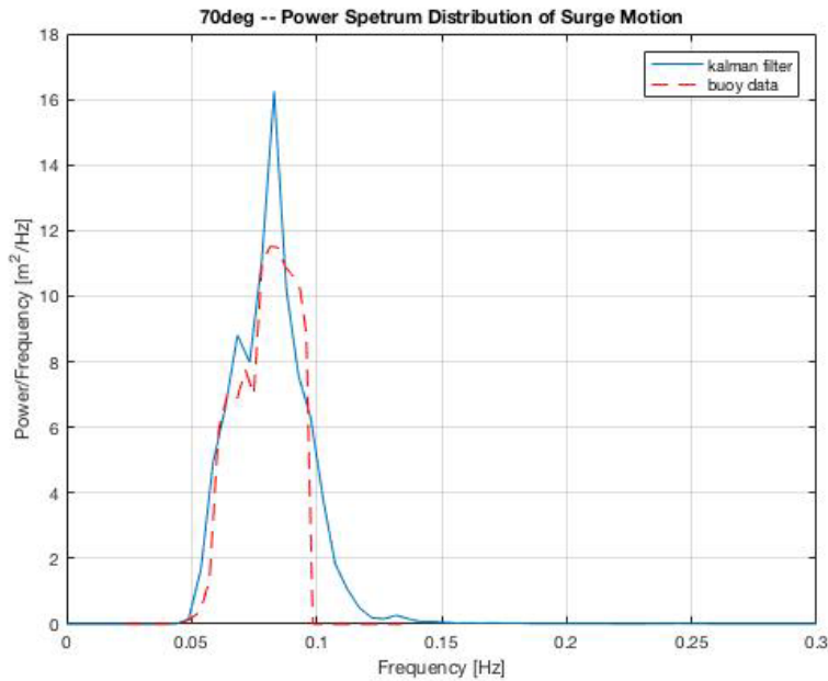
Fig. 5 Surge motion PSD at heading angle of 70°
