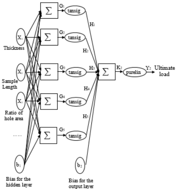
Fig. 4 ANN architecture
