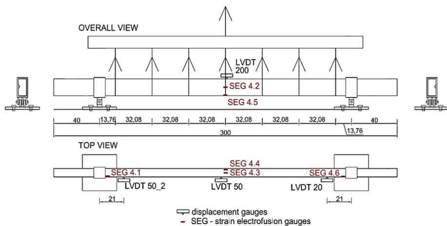
Fig. 5 Scheme of laboratory stand
