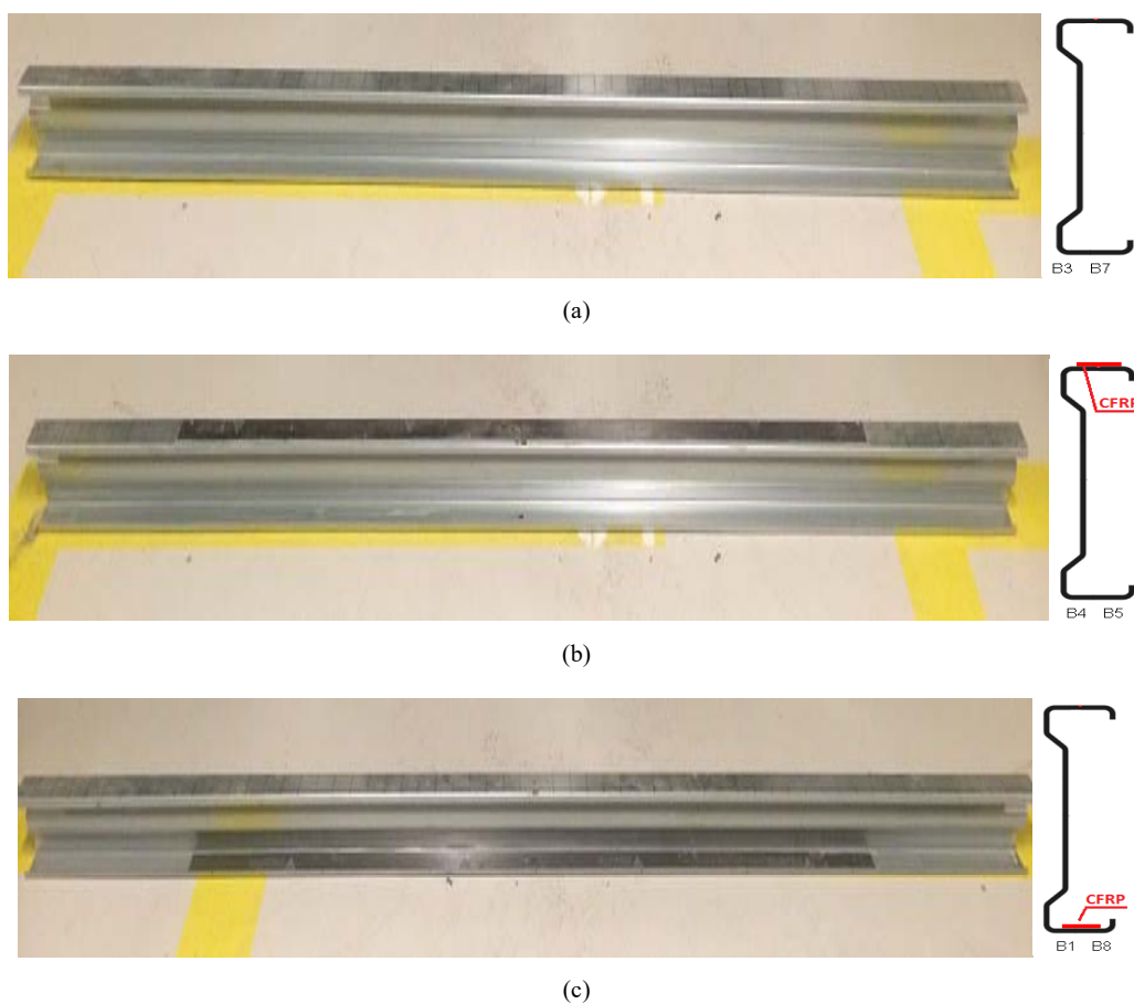
Fig. 6 CFRP tape location (a) B7 and B3; (b) B1 and B8; (c) B4 and B5
