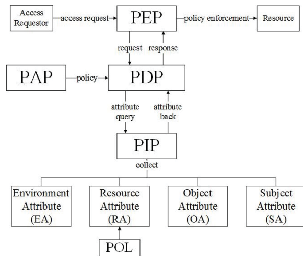
Fig. 3 Architecture of PABAC model
