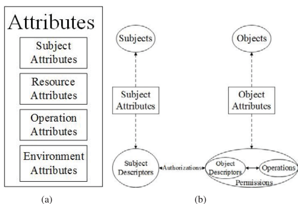
Fig. 1 (a) Relations of attributes. (b) Architecture of ABAC
