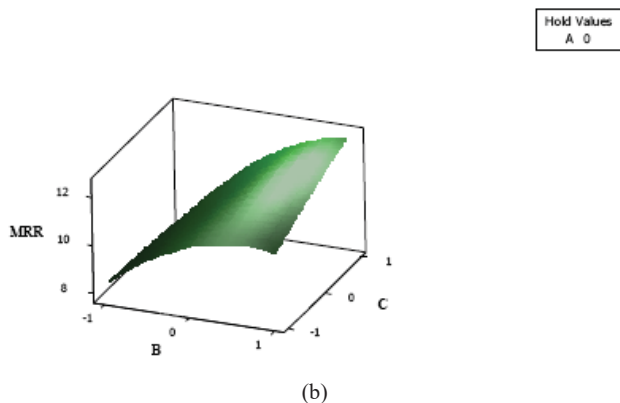
Fig. 1 Response surface plots of MRR for significant interactions (a). I x T on (b) T on x T off
