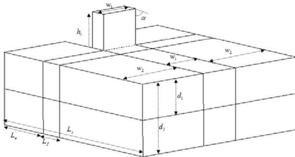
Fig. 2 Parameters of the FE model
