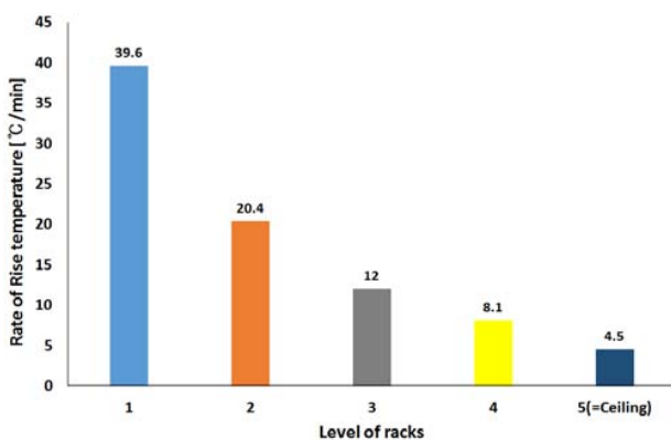
Fig. 9 The rate of temperature rise per minute
