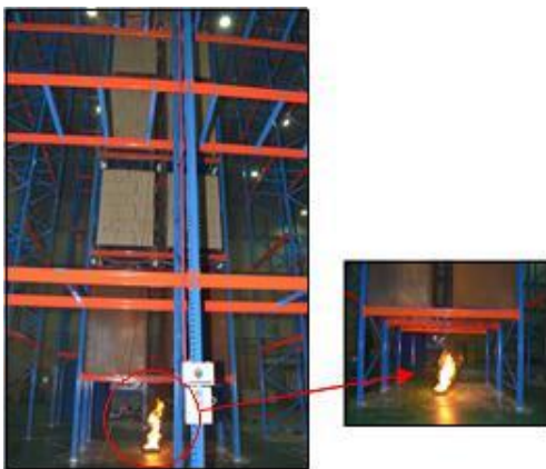
Fig. 7 The n-heptane fire experiment
