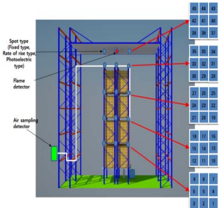
Fig. 1 Schematic of fire detector arrangement
