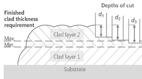
Fig. 1 Determining the levels for depth of cut
