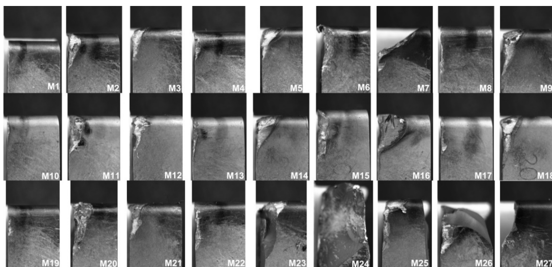
Fig. 3 Flank wear on inserts from test M1 to M27
