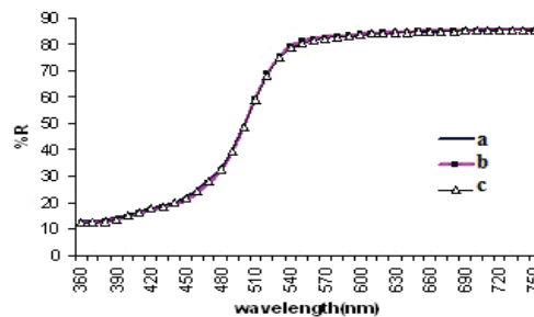
Fig. 5 The R% graph samples dyed with of untreated and plasma treated Reactive yellow 105 with plasma at 1 and 5 minutes of plasma exposure time
