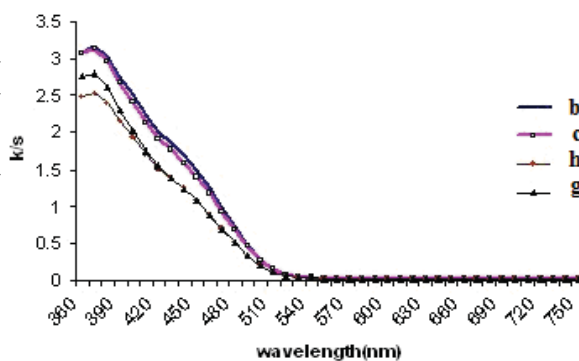
Fig. 6 The K/S rate of samples dyed with plasma treated Reactive yellow 105 at one and 5 minutes of plasma exposure time before and after washing
