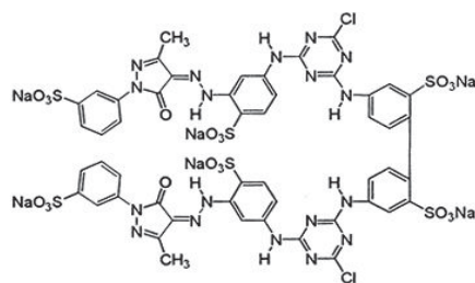
Fig. 2 Molecular structure of reactive dye named Reactive yellow 105(C 50 H 32 Cl 2 N 18 Na 6 O 20 S 6 )
