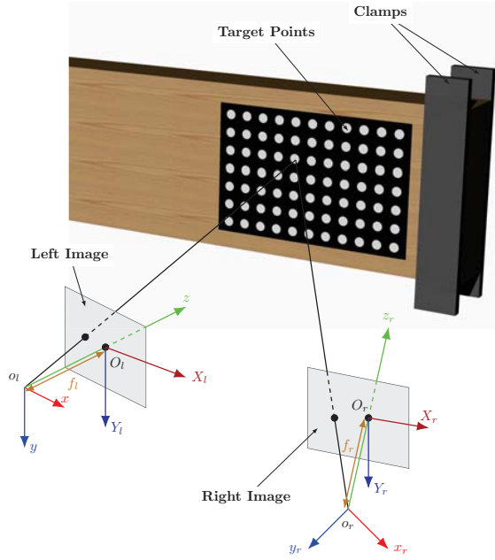
Fig. 1 Target points reconstruction of binocular stereo vision
