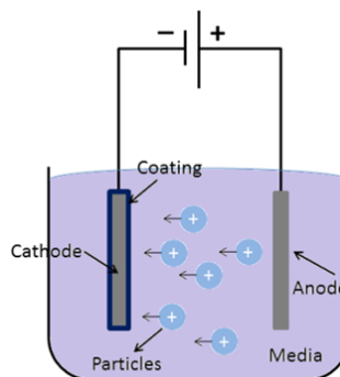
Fig. 2 Schematic image of the EPD cell
