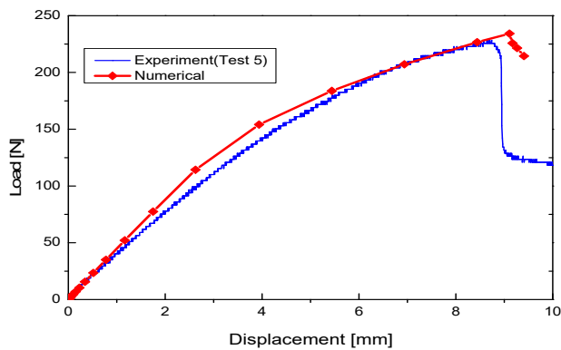
Fig. 7 Load-midspan deflection responses
