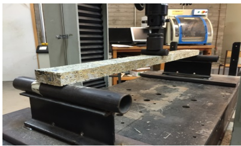
Fig. 2 Three-point bending test: (a) geometric and loading characteristics, (b) Test setup. Dimensions in mm
