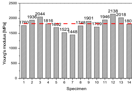
Fig. 4 Comparison of MOE
