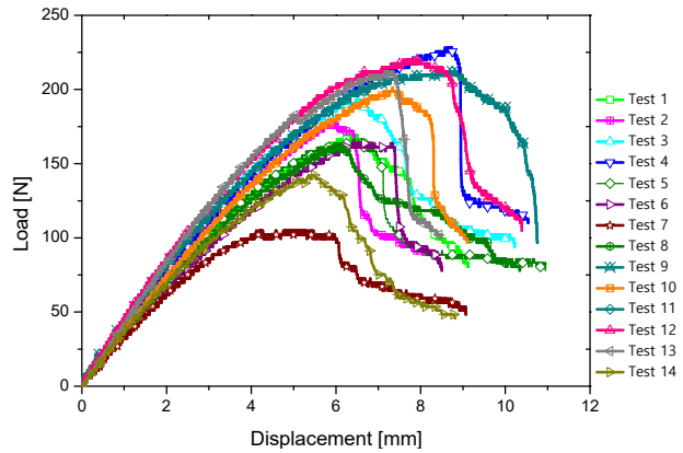
Fig. 3 Load displacement curves for beams
