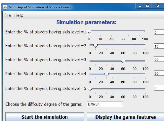
Fig. 6 The Simulator Interface
