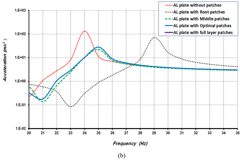
Fig. 3 Numerical FRF of the plate at different patch locations: (a) First bending mode, (b) Second bending mode
