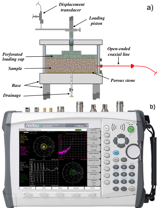
Fig. 1 Experimental setup of the relative subsidence test apparatus (a) and VNA Master MS207C network analyser (b)
