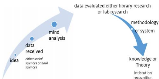
Fig. 3 Data process
