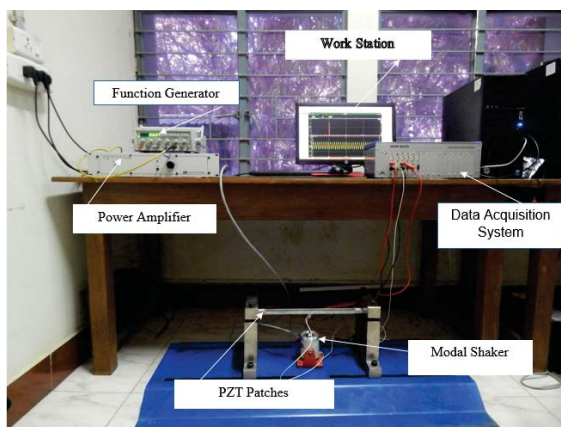
Fig. 7 Experimental set up of Fixed-Fixed beam with PZT Patch
