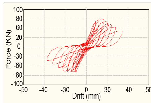
Fig. 5 Load-Drift Responses
