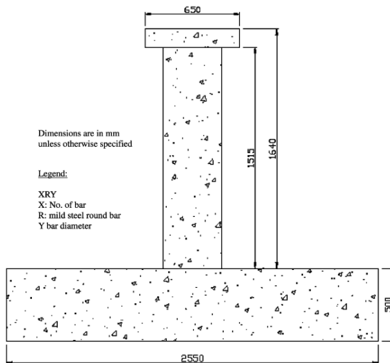
Fig. 2 Reinforced Concrete Details in the Test Samples [7]
